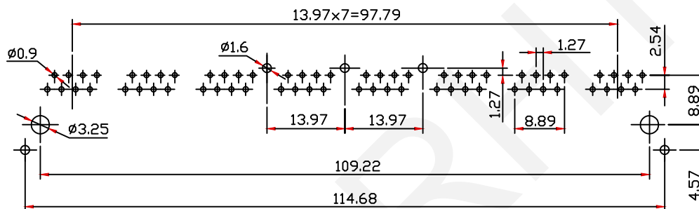
PCB Layout
